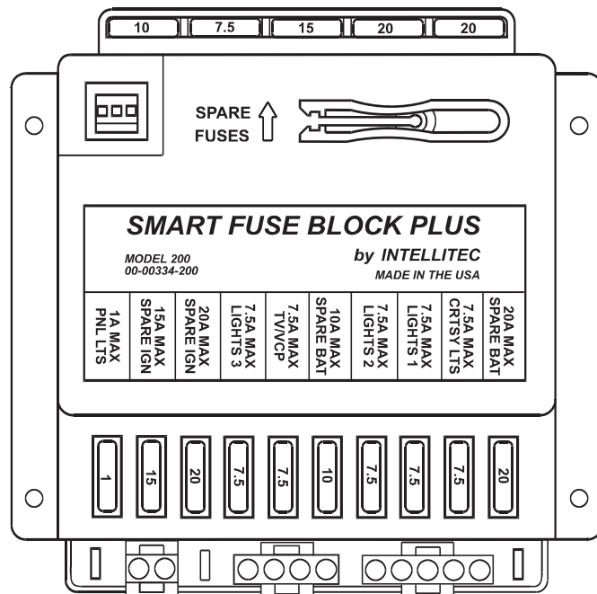
Part Number 00-00334-200
